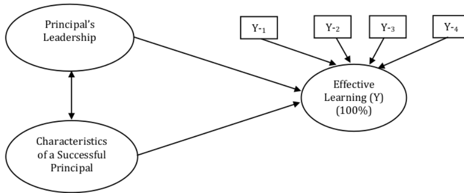
Figure 1. Y latent variables measured by indicators Y-1, Y-2, Y-3 and Y-4
